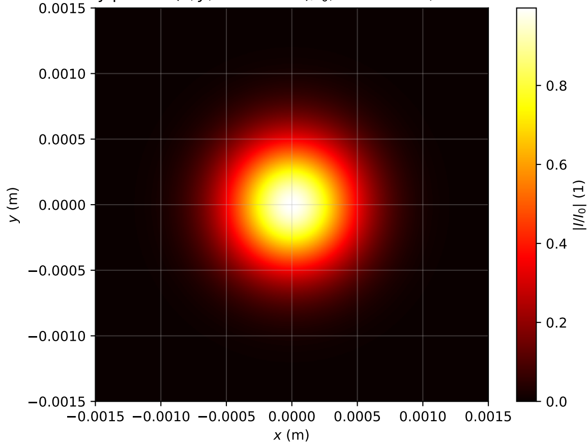
Intensity profile I(x, y, z = 0.557m)/I_0 , Pin=0.3Pcr, artificial time
